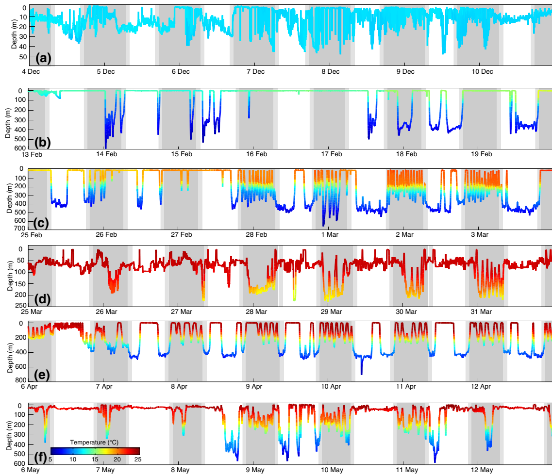
Fig. 5 One week time series of depth ( line ) and temperature ( color ) for white shark 18-F, 2004–2005 a nearshore, off the Farallon Islands, California, b traveling west through the California Current, c traveling
